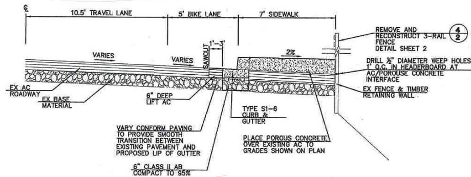
TYPICAL SECTION IN AREA WITH RETAINING WALLS
