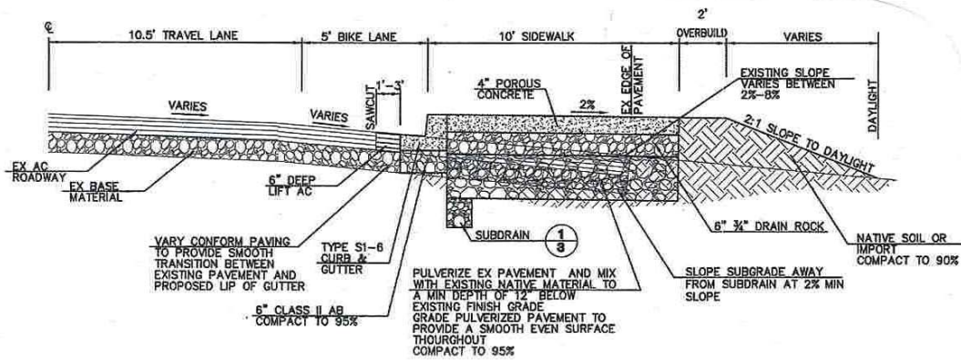
TYPICAL SECTION IN AREAS WITHOUT RETAINING WALLS
